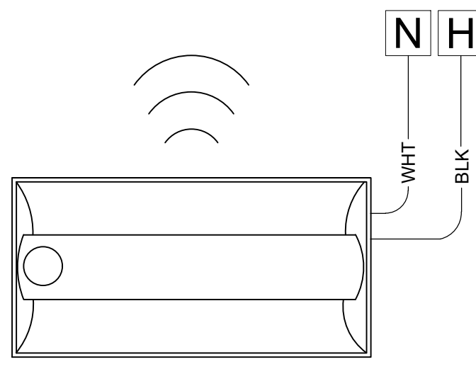
2VTL4 rES7PDT GENERAL LIGHTING
